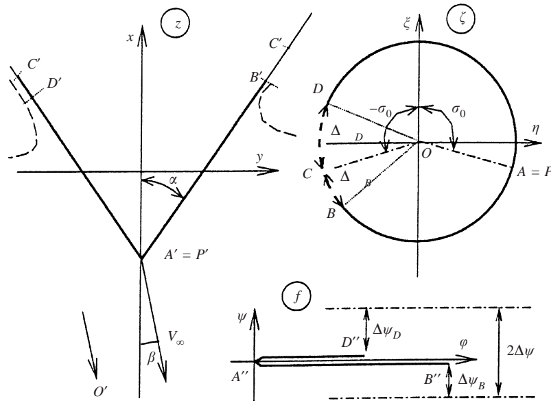
FIGURE 2. Conformal mapping (attached flow).
