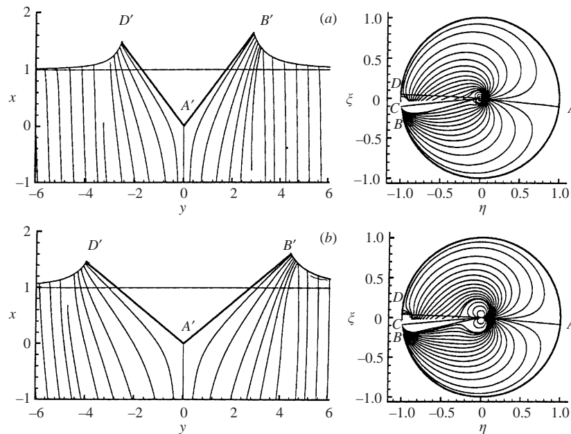
FIGURE 7. Unsymmetrical attached flow field: iso- \psi line distributions in the physical and in the transformed plane, \alpha = 60^\circ , \beta = 4^\circ (a); \alpha = 70^\circ , \beta = 4^\circ (b).
