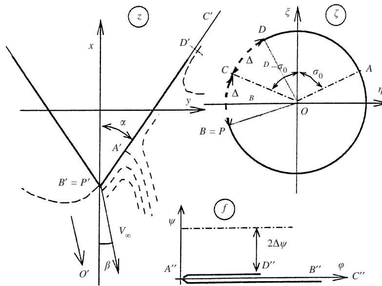
FIGURE 3. Conformal mapping (separated flow).
