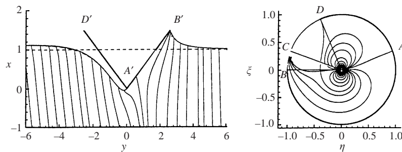
FIGURE 9. Separated flow field. \alpha = 60^\circ and \beta = 10^\circ : iso- \psi line distributions in the physical and in the transformed plane.
