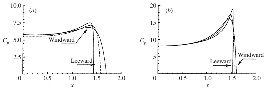
FIGURE 8. Pressure distribution for attached flow, \alpha = 60^\circ (a), \alpha = 70^\circ (b), \beta = 0 (dashed lines), \beta = 4^\circ (continuous lines).
