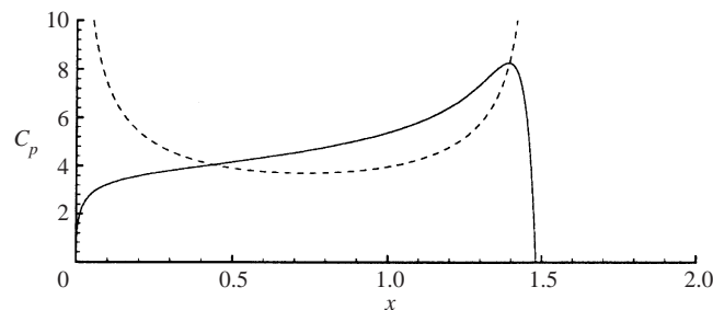
FIGURE 10. Pressure distribution for the separated flow, \alpha = 60^\circ , \beta = 10^\circ : von Kármán's theory (dashed line), present method (continuous line).
