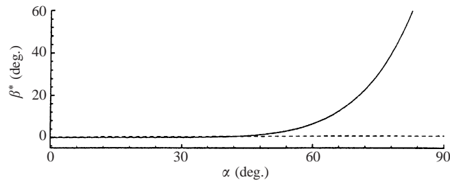
FIGURE 6. Values of the sideslip angle for the onset of separation \beta^* vs. the wedge angle \alpha . Above the line the flow separates from one side.
