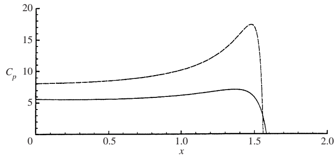
FIGURE 5. Symmetrical pressure distribution, \alpha = 60^\circ (continuous line), \alpha = 70^\circ (dashed line).
