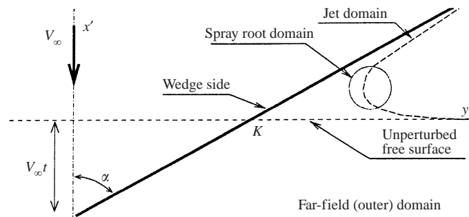
FIGURE 1. Proposed subdomains.
