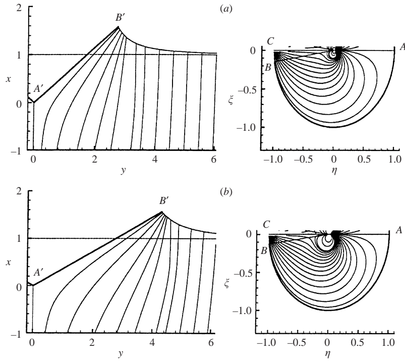
FIGURE 4. Symmetrical flow field, \alpha = 60^\circ (a), \alpha = 70^\circ (b).
